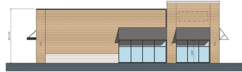
Bldg. B - West Elevation 1/8" = 1'-0"
